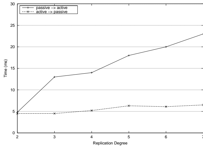
Figure 6: Strategy switching cost as a function of the replication degree
