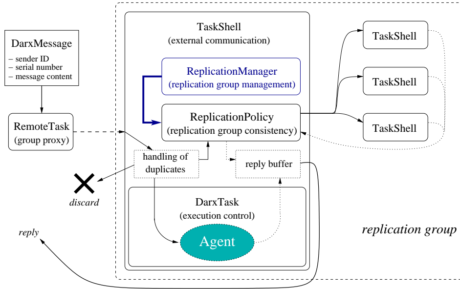
Figure 2: Replication management scheme
