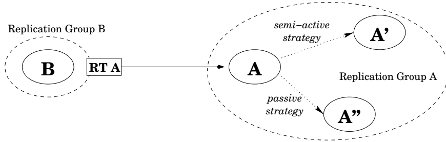
Figure 3: A simple agent application example
