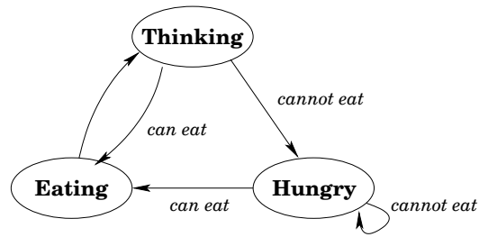
Figure 4: Dining philosophers over DARX: state diagram
