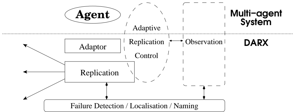
Figure 1: DARX application architecture
