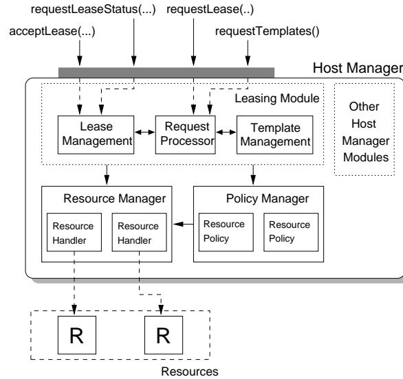
FIG. 3.1. Components within the Host Manager.
