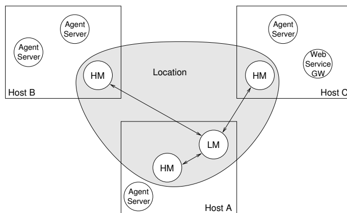
FIG. 4.1. Overview of an AgentScape location.
