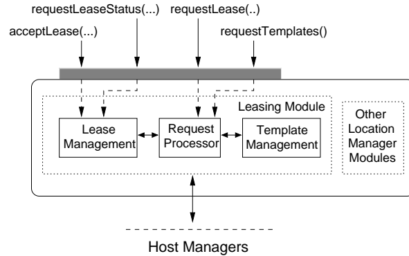
FIG. 3.2. Leasing components within the domain coordinator.
