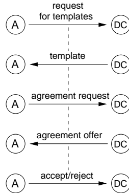
FIG. 2.4. Extended WS-Agreement protocol.
